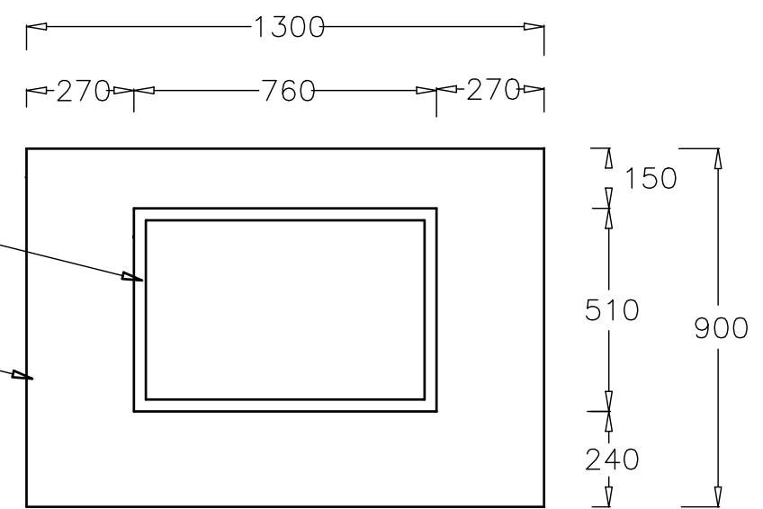
TYPE A2 – SIDE ENTRY PIT PRECAST CONCRETE LID & SURROUND
